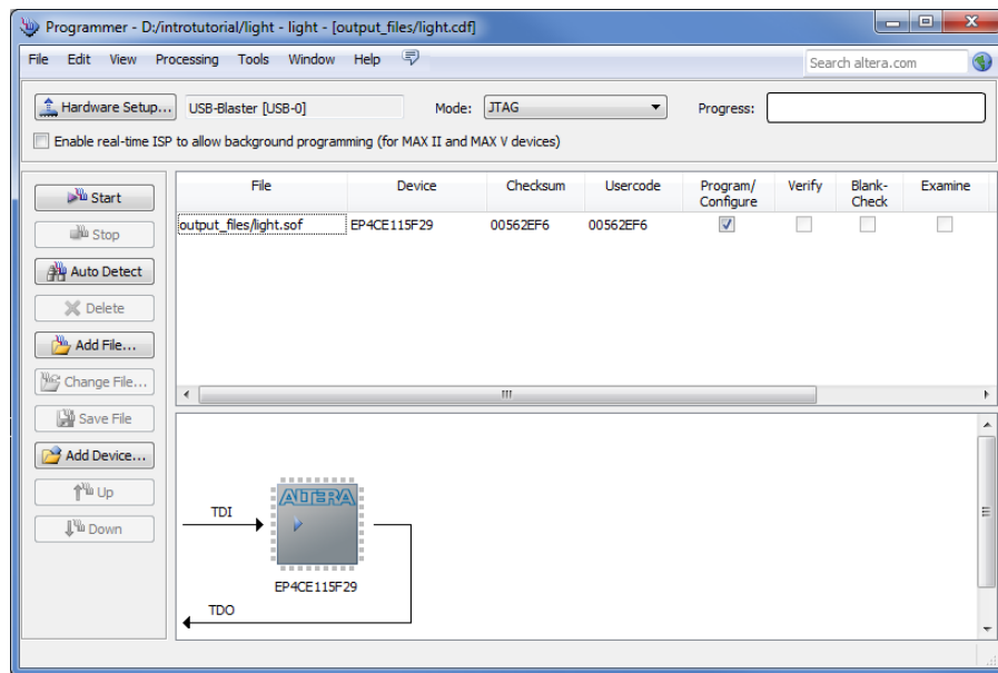
Figure 37. The Programmer window.
