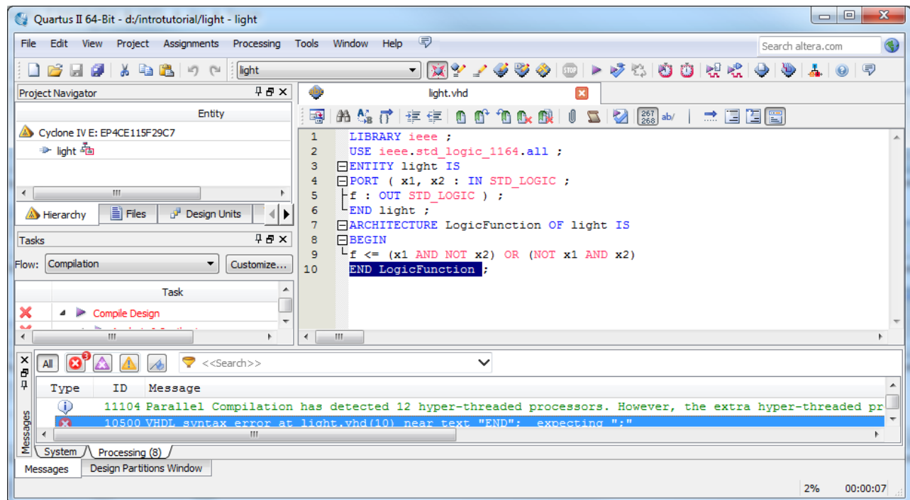
Figure 22. Identifying the location of the error.
