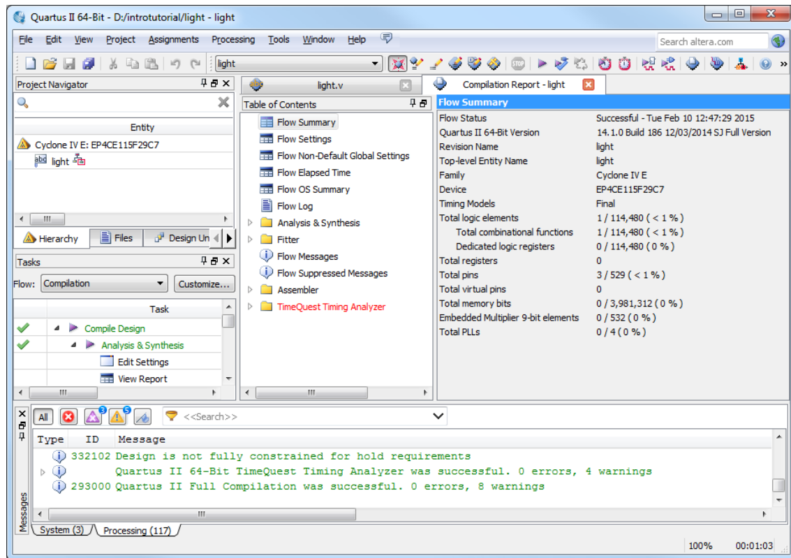
Figure 19. Display after a successful compilation.
