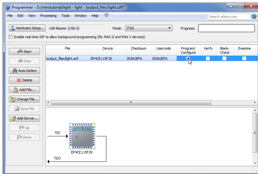
Figure 39. The updated Programmer window.
