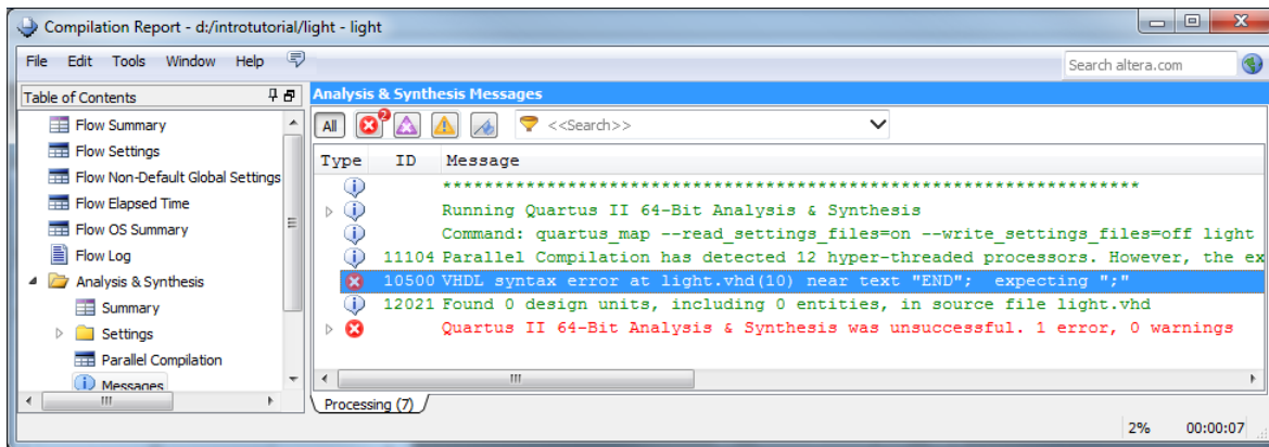
Figure 21. Error messages.
